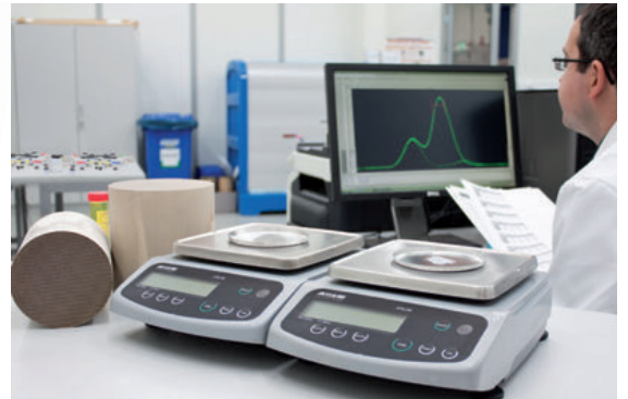
Laboratory assessment of HJS blu@mission ® vs. low-budget catalytic converters
